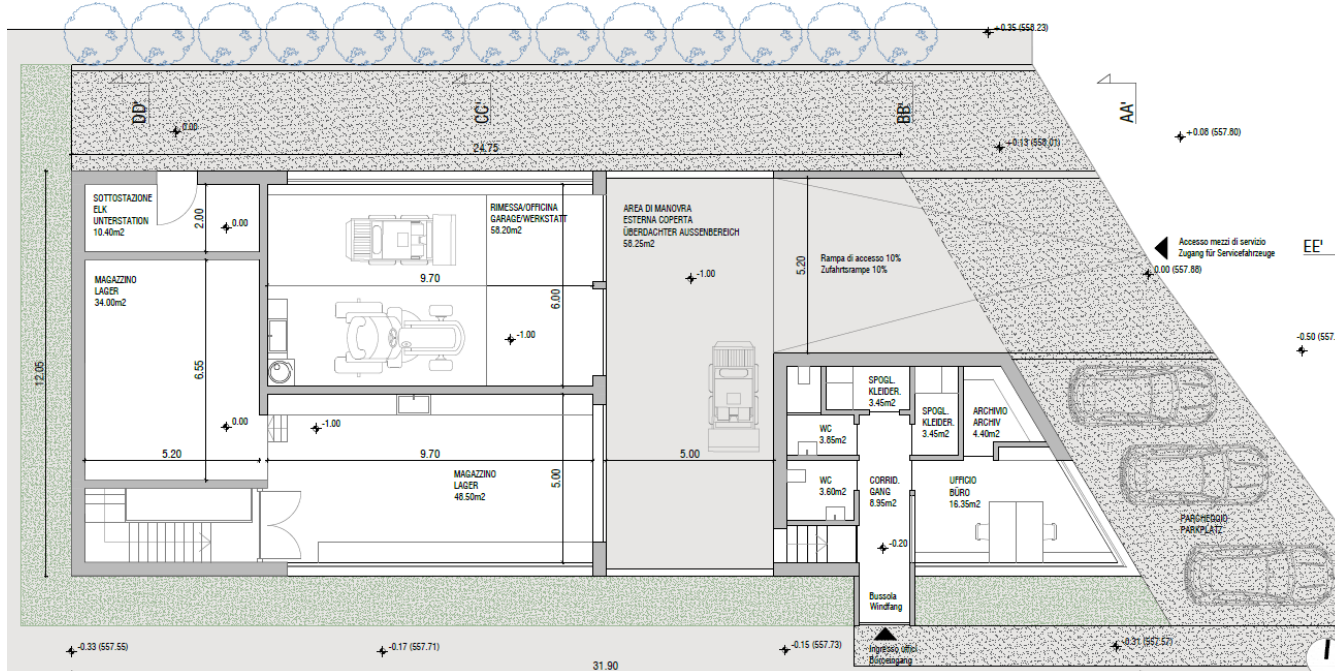
ERDGESCHOSS | PIANO TERRA
